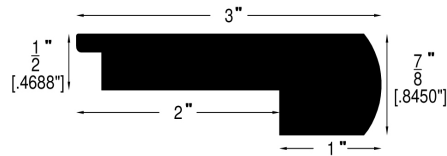
Stair Nose (712)
