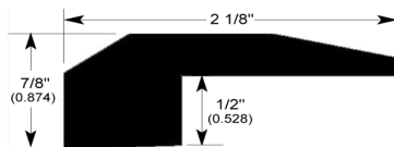
Threshold 7/16 - 3/4 (011)
