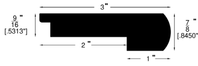
Stair Nose (721)
