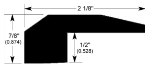
Threshold 7/16 - 3/4 (011)
