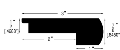
Stair Nose (712)
