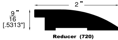
Reducer (720)
