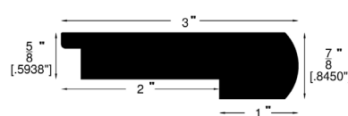
Stair Nose (738)
